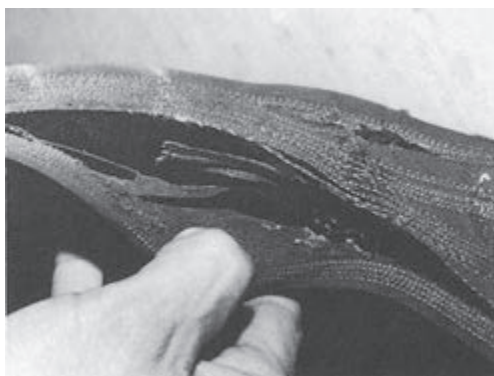
An example of Casing Break Up (CBU) in a bias tire at the lower sidewall caused by running the tire at pressures below those recommended.
